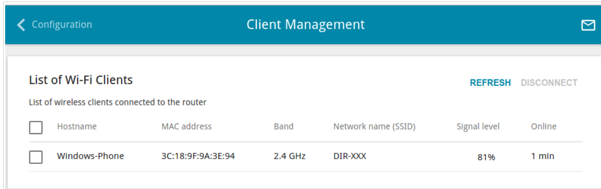
Figure 100. The page for managing the wireless clients.
