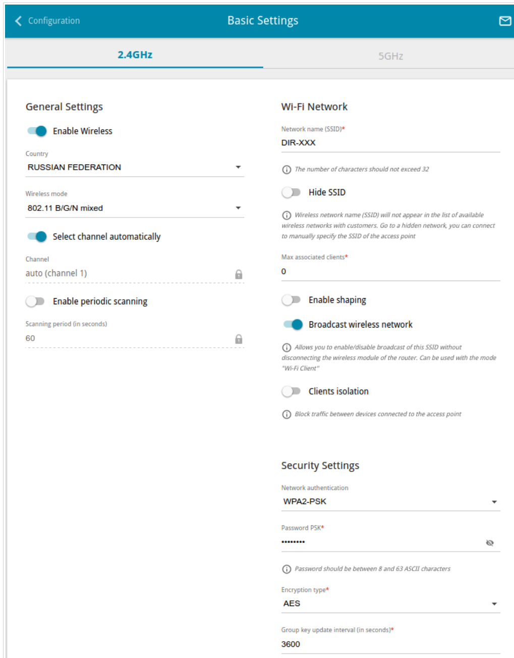
Figure 94. Basic settings of the wireless LAN in the 2.4GHz band.
