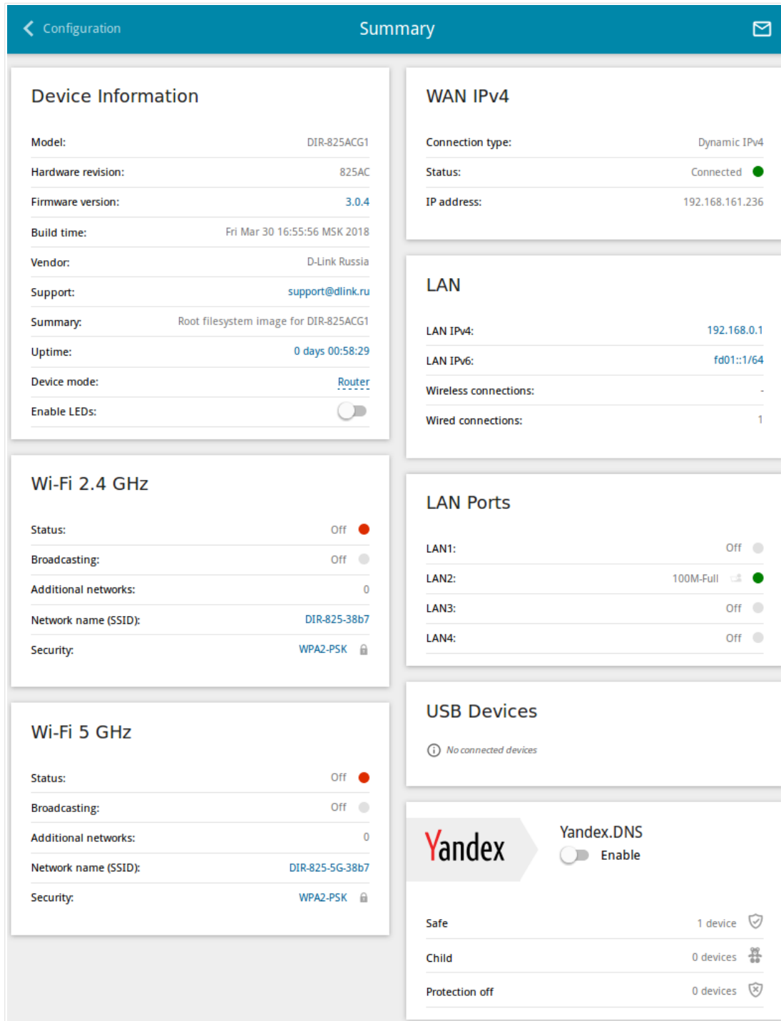
Figure 15. The summary page.
