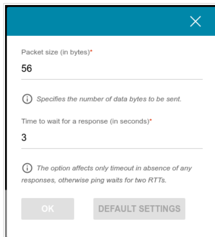
Figure 170. The System / Ping page. The additional settings window.
