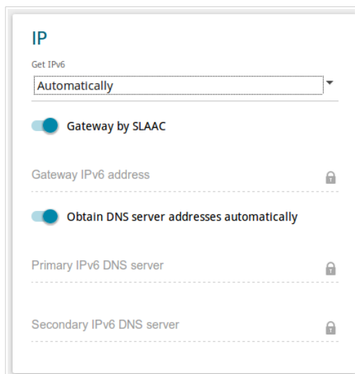
Figure 77. The page for creating a new PPPoE Pv6 connection. The IP section.
