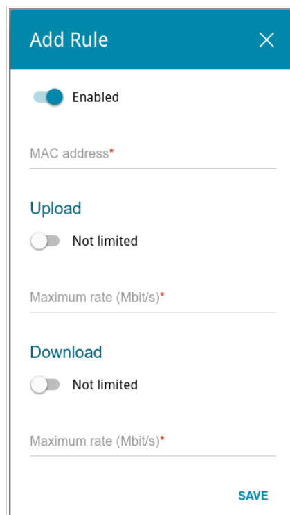
Figure 106. The window for setting up rate limit.
