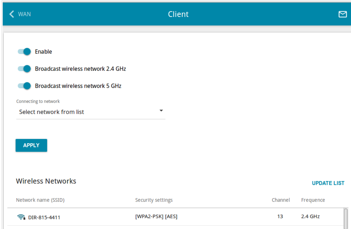
Figure 104. The page for configuring the client mode.
