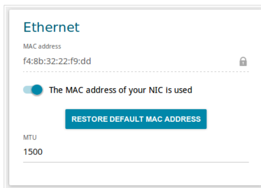
Figure 75. The page for creating a new PPPoE IPv6 connection. The Ethernet section.
