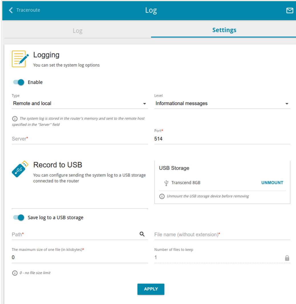
Figure 167. The System / Log page. The Settings tab.
