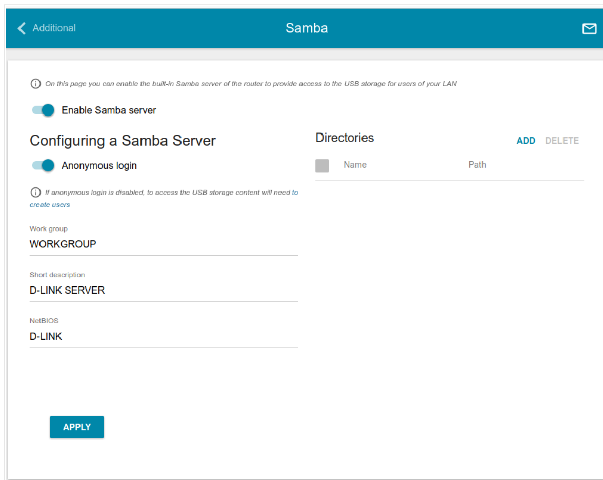
Figure 115. The USB Storage / Samba page.
