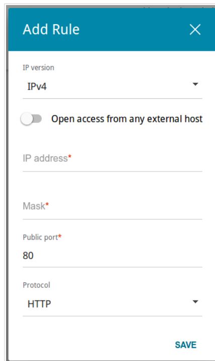
Figure 146. The window for adding a rule for remote management.
