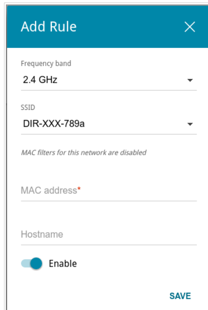
Figure 109. The window for adding a rule for the MAC filter.
