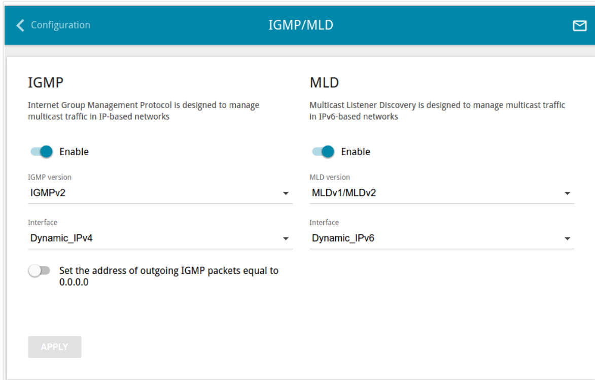
Figure 150. The Advanced / IGMP/MLD page.
