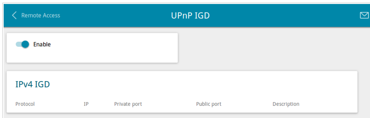
Figure 147. The Advanced / UPnP IGD page.
