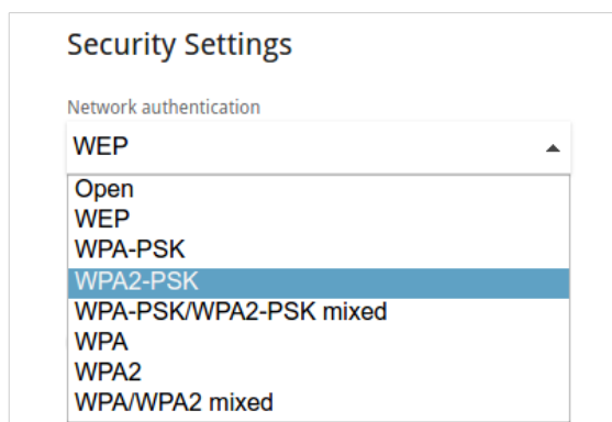
Figure 96. Network authentication types supported by the router.
