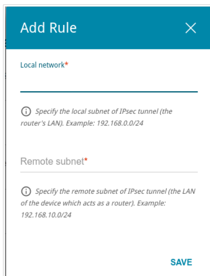
Figure 155. The page for adding an IPsec tunnel. The window for adding a tunneled network.
