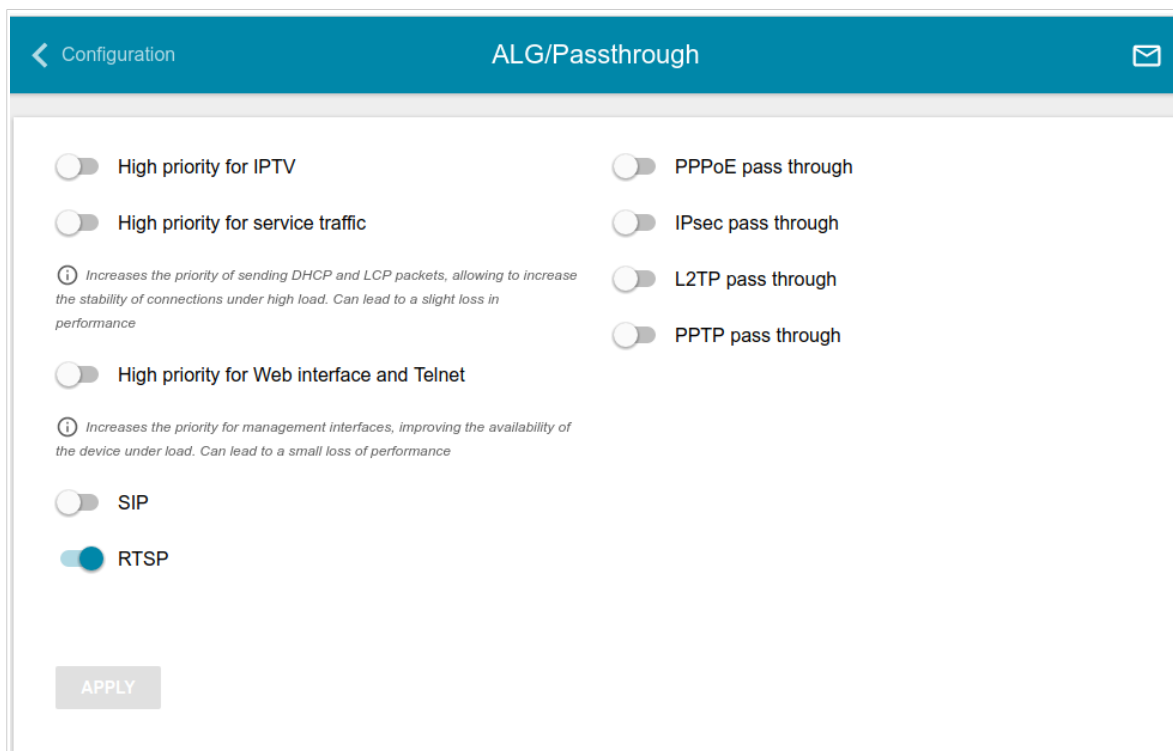
Figure 151. The Advanced / ALG/Passthrough page.
